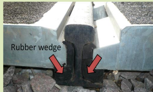
Rubber wedge
