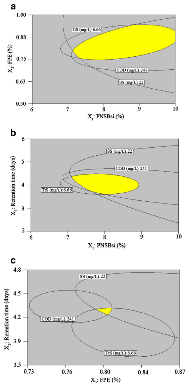
Fig. 2. The overlay interaction plots of two variables: stimulated indigenous purple non sulfur bacteria (PNSBsi) and fermented pineapple extract (FPE) (a), PNSBsi and retention time (RT) (b), FPE and RT (c) on the efficiency to treat non sterile rubber sheet wastewater under microaerobic light conditions.
