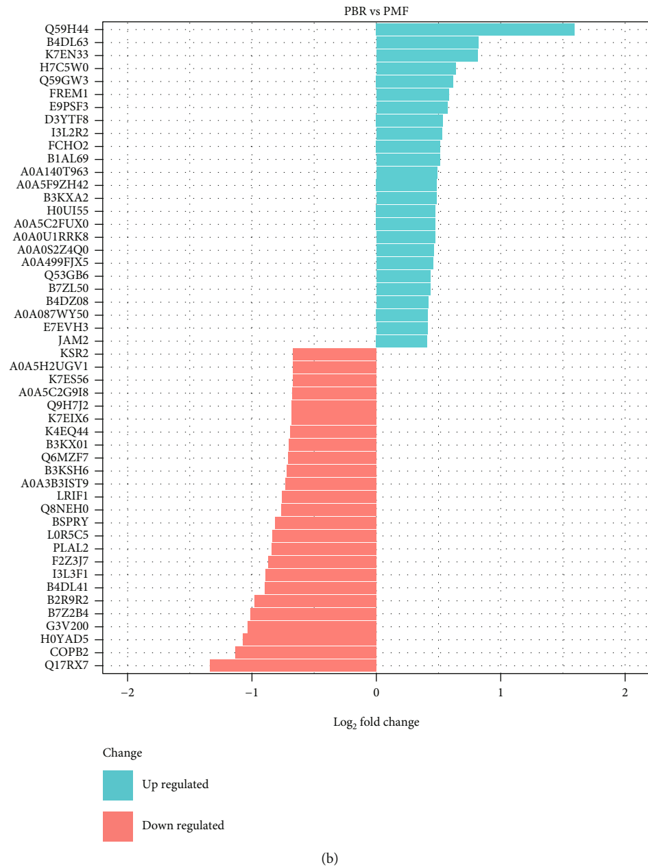
FIGURE 9: Top 10 differentially expressed proteins in HCT (a) and PMF (b) cells.
