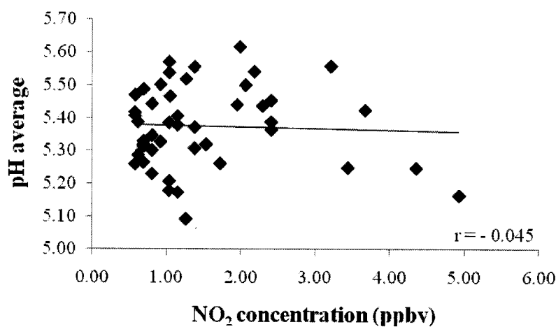
Figure 4.37 Correlation between NO 2 in the rainy season and average pH of barks.
