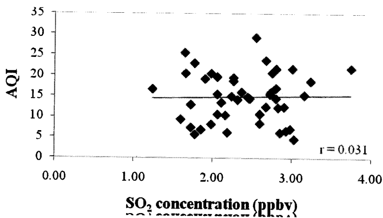
Figure 4.36 Correlation between SO 2 in the winter season and AQI.
