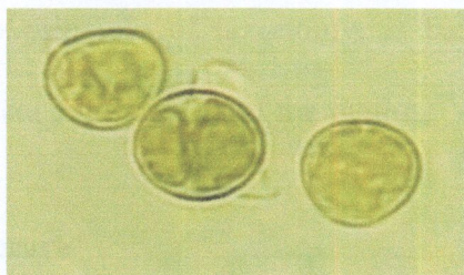
Figure 2.6 Single cells of Trebouxia , the most common green alga found in lichens.
