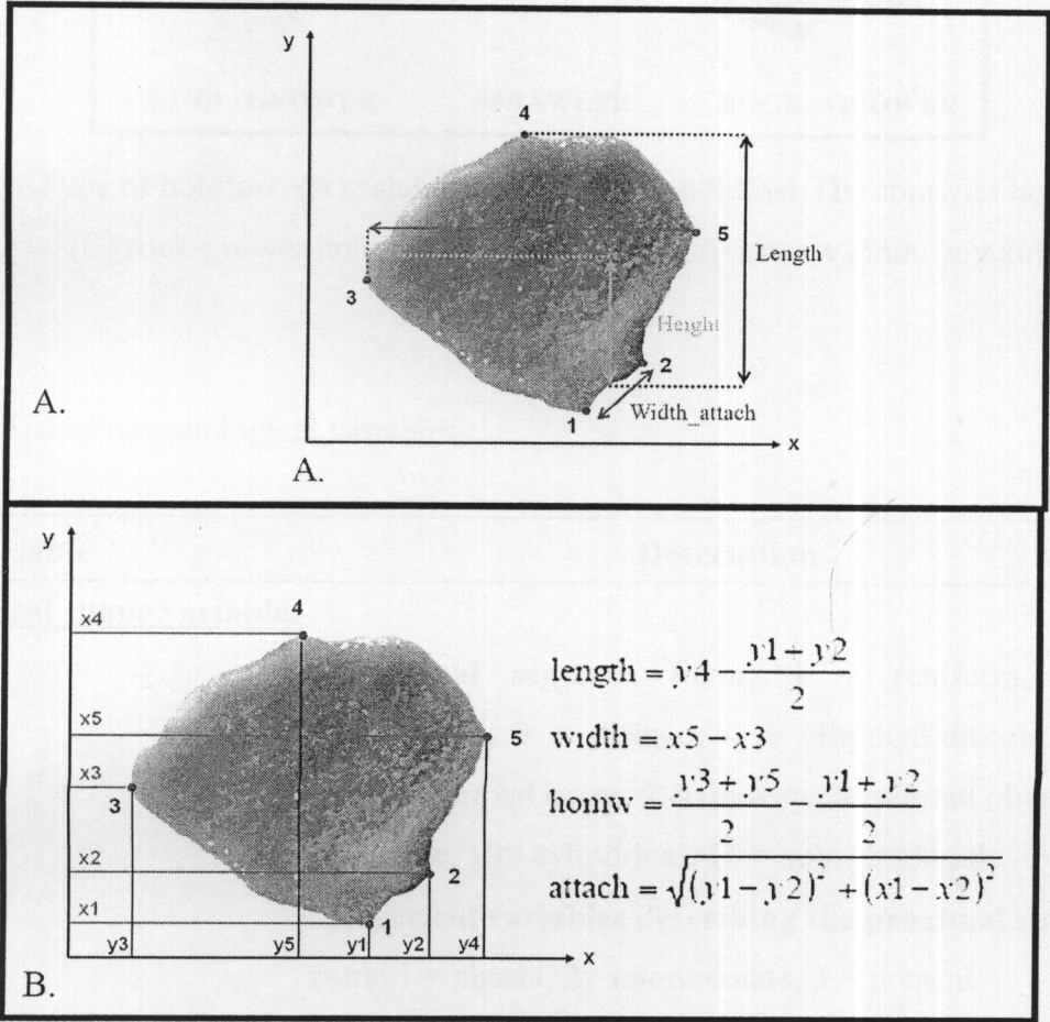
Figure 12 Segment Morphological: (A) conventional measurement, (B) five landmarks of segment and equations for calculated (modified from Verbruggen et al. , 2005a)
