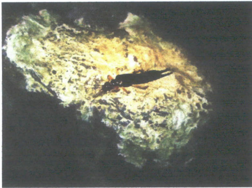
Dermaptera: earwigs
