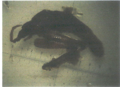
Orthoptera: grasshoppers
