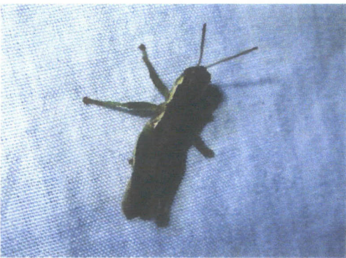
Orthoptera: grasshoppers
