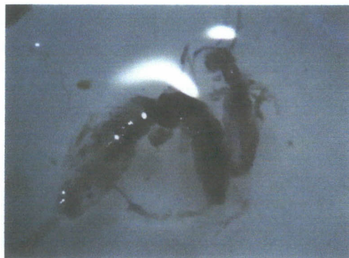
Collembola: springtails
