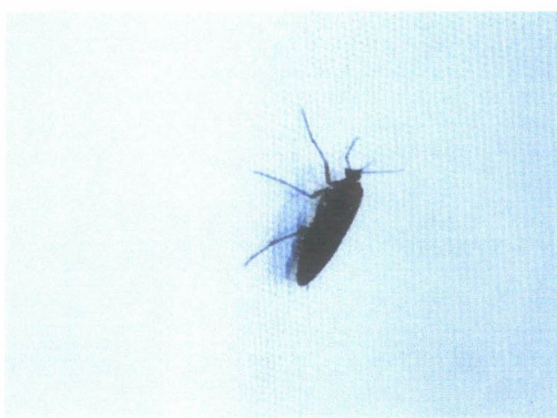
Diptera: flies
