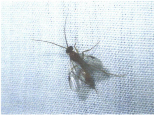
Hymenoptera-Non Formocidae
