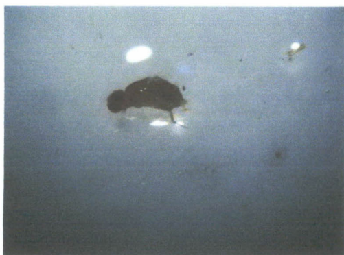
Diptera: flies
