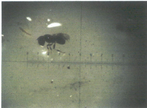
Hymenoptera: Non-Fornicidae
