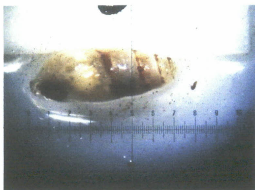
Gastropoda
