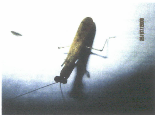
Mantodea: mantids
