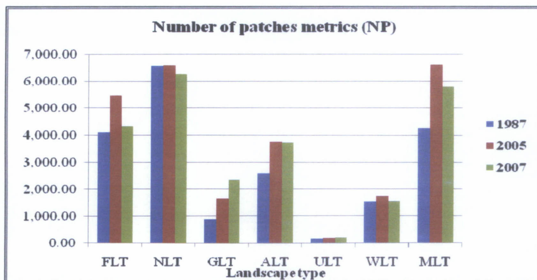
Figure 6.9 Comparison of number of patch among 1987, 2005 and 2007 in the study area.
