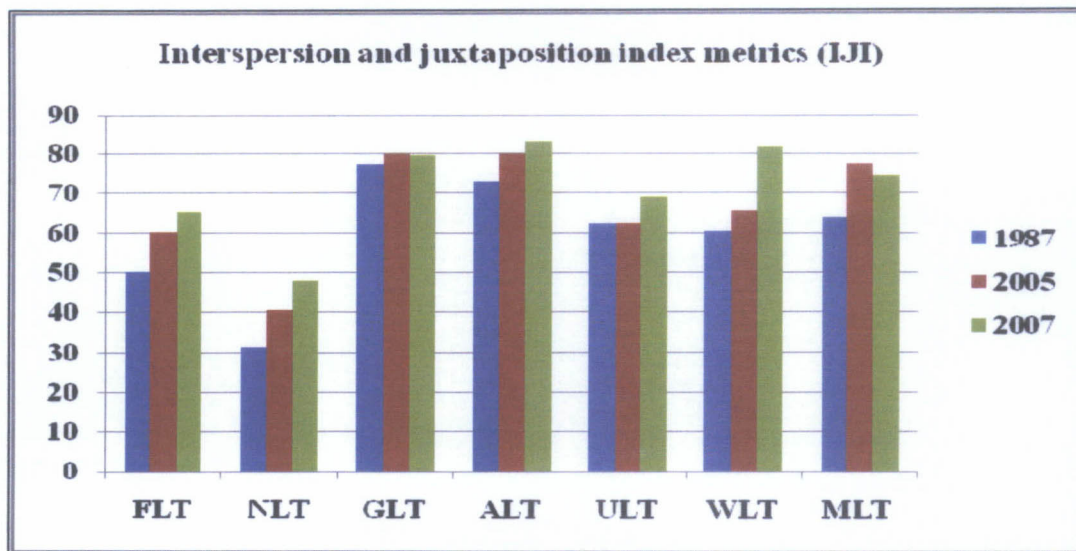
Figure 6.21 Comparison of Interspersion and juxtaposition index among 1987, 2005 and 2007 in the Thap Lan National Park.
