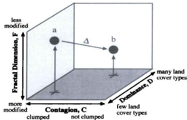
Figure 4.2 Landscape Metric Feature Space (Jensen, 2007).
