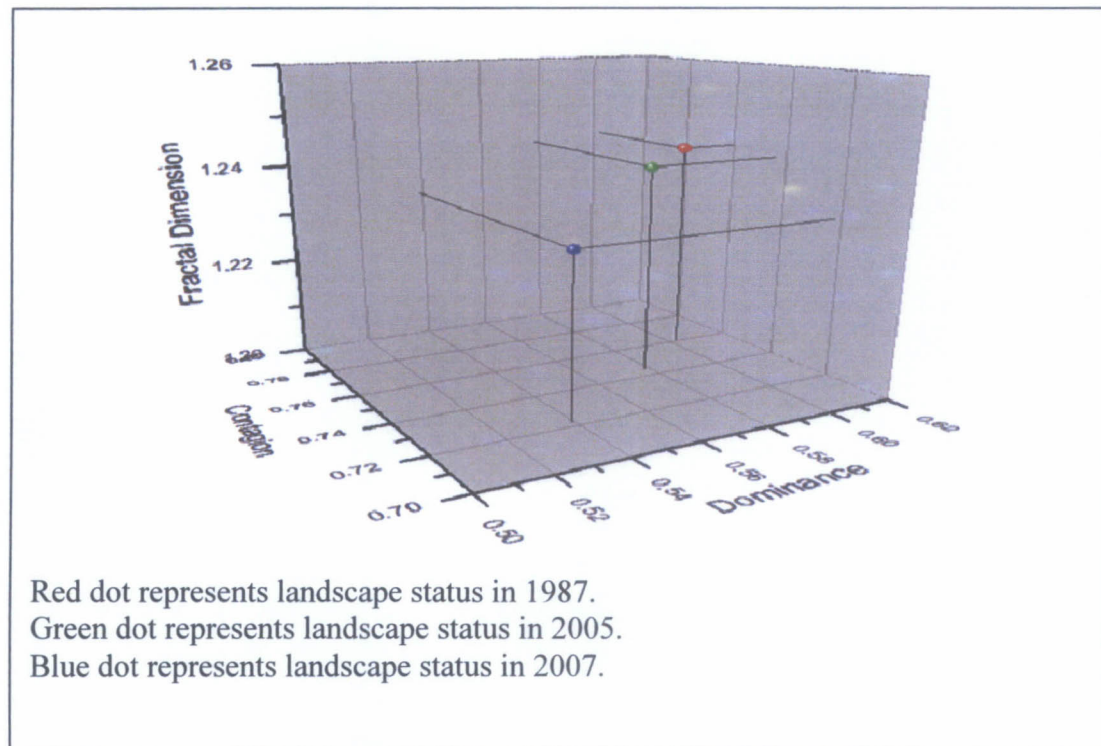
Figure 6.7 Three dimensional landscape metric feature space and their changes of the Thap Lan National Park.
