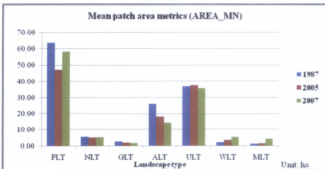
Figure 6.11 Comparison of mean patch area among 1987, 2005 and 2007 in the study area.
