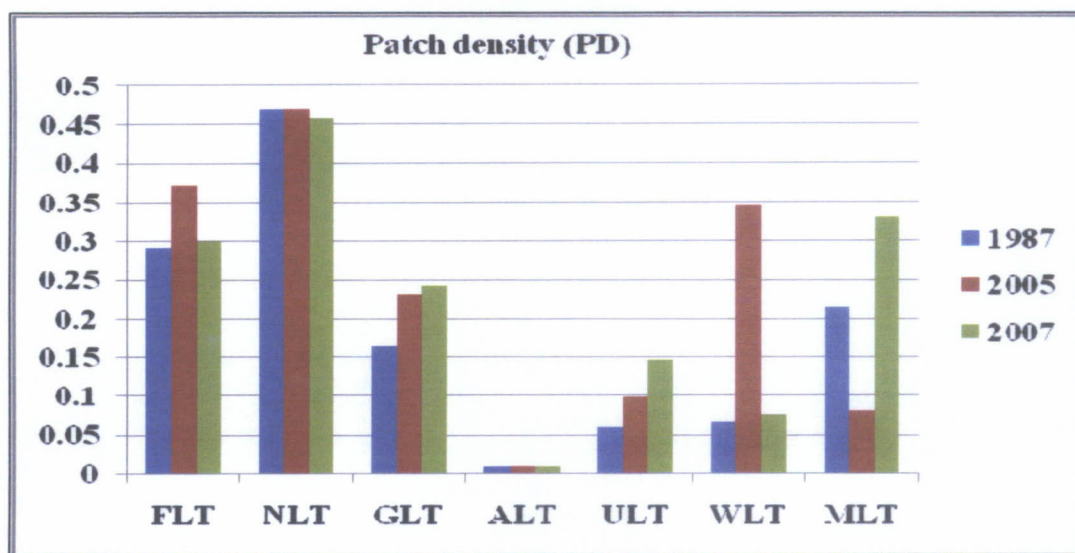
Figure 6.17 Comparison of patch density among 1987, 2005 and 2007 in Thap Lan National Park.
