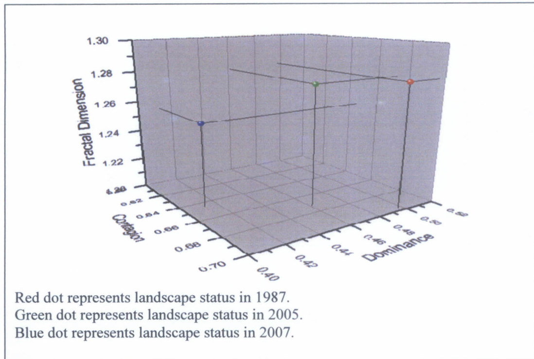
Figure 6.6 Three dimensional landscape metric feature space and their changes of the Thap Lan National Park and its 5 km buffer.
