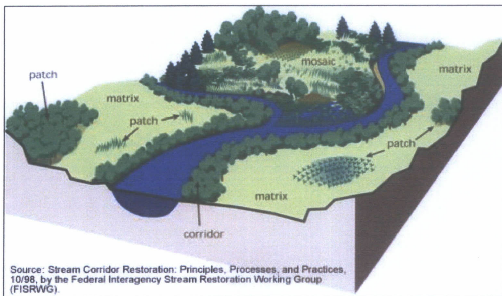
Figure 2.1 Three main components of landscape: matrix, patch and corridor.
