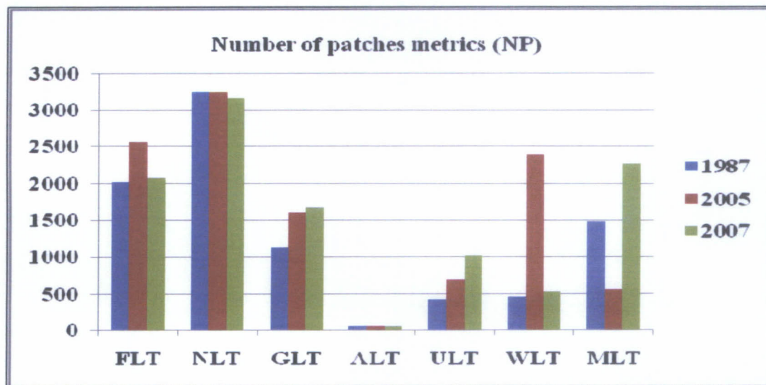
Figure 6.16 Comparison of number of patch among 1987, 2005 and 2007 in Thap Lan National Park.
