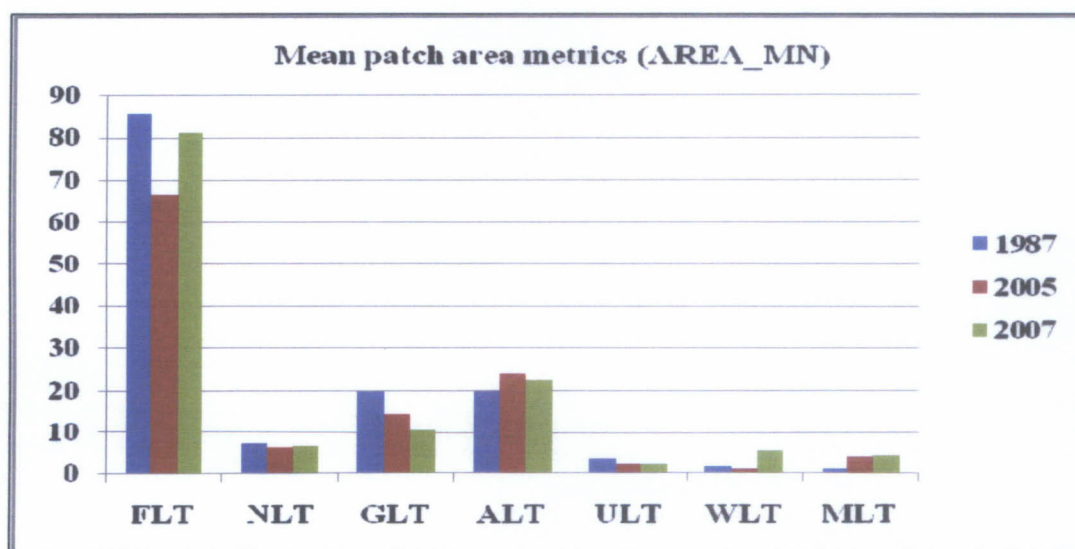
Figure 6.18 Comparison of mean patch area among 1987, 2005 and 2007 in Thap Lan National Park.
