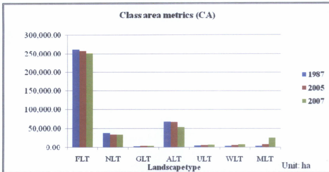
Figure 6.8 Comparison of class area among 1987, 2005 and 2007 in the study area.
