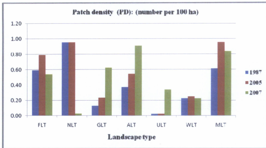
Figure 6.10 Comparison of patch density among 1987, 2005 and 2007 in the study area.
