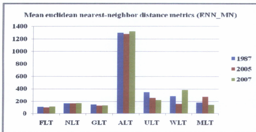
Figure 6.20 Comparison of Mean Euclidean nearest-neighbor distance among 1987, 2005 and 2007 in Thap Lan National Park.
