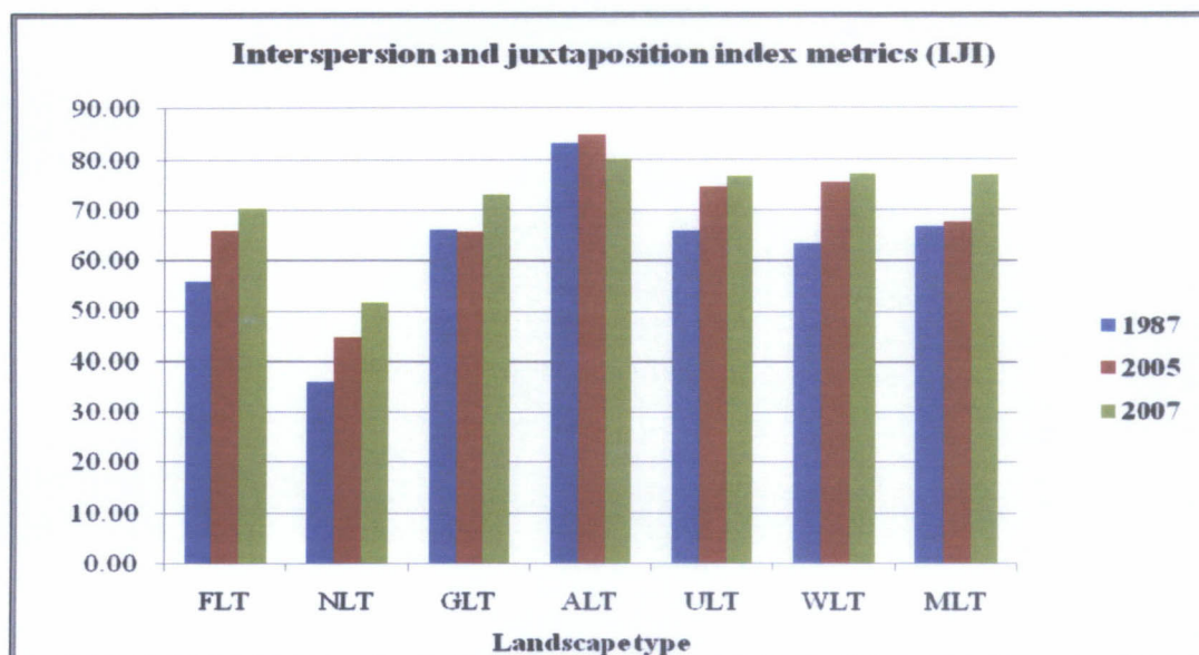
Figure 6.14 Comparison of Interspersion and juxtaposition index among 1987, 2005 and 2007 in the study area.
