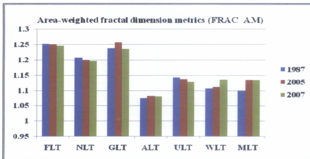
Figure 6.19 Comparison of Area-weighted fractal dimension among 1987, 2005 and 2007 in Thap Lan National Park.
