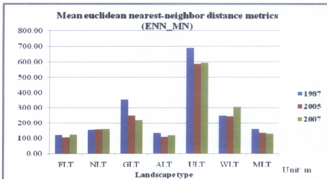
Figure 6.13 Comparison of Mean Euclidean nearest-neighbor distance among 1987, 2005 and 2007 in the study area.
