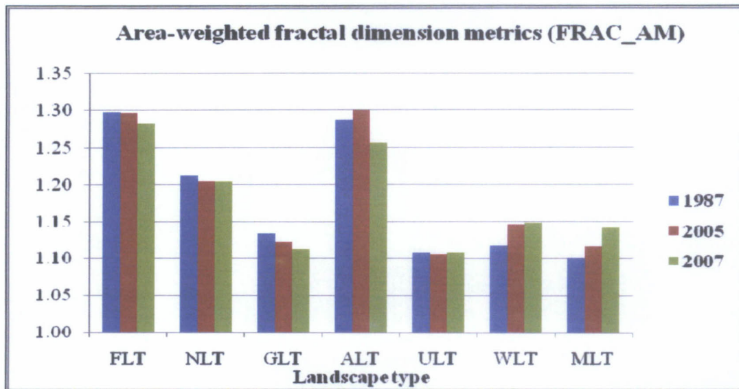
Figure 6.12 Comparison of Area-weighted fractal dimension among 1987, 2005 and 2007 in the study area.
