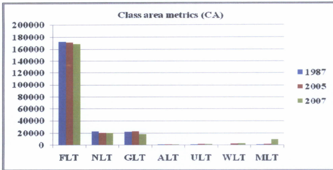
Figure 6.15 Comparison of class area among 1987, 2005 and 2007 in Thap Lan National Park.
